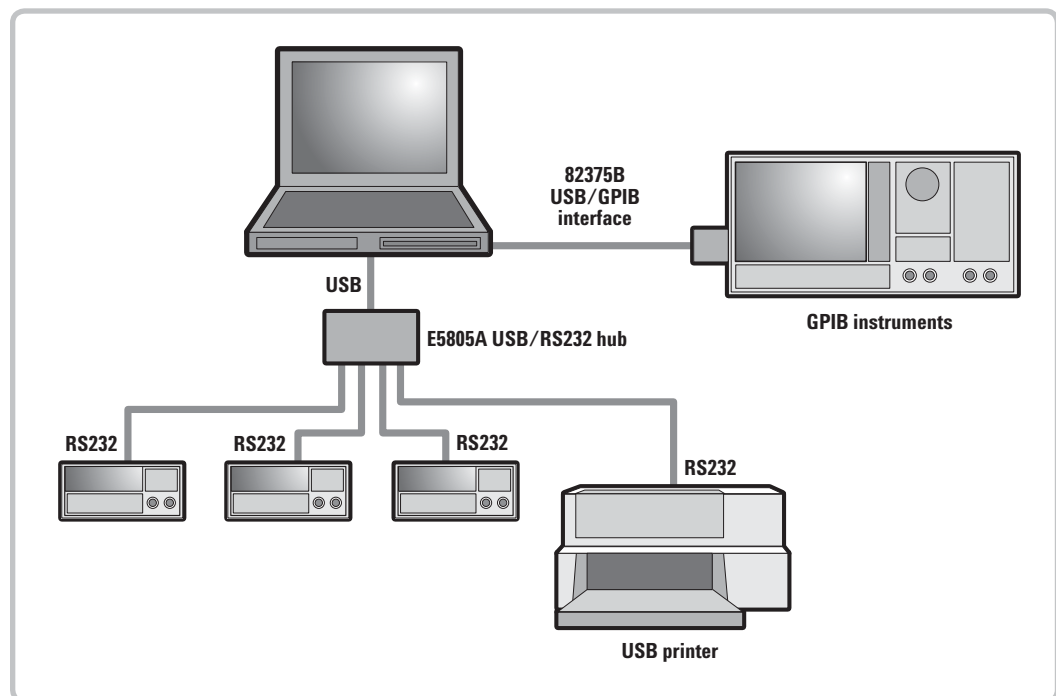
Figure 2. A self-powered USB hub makes it easy to create a hot-pluggable system that anyone can connect to and use
