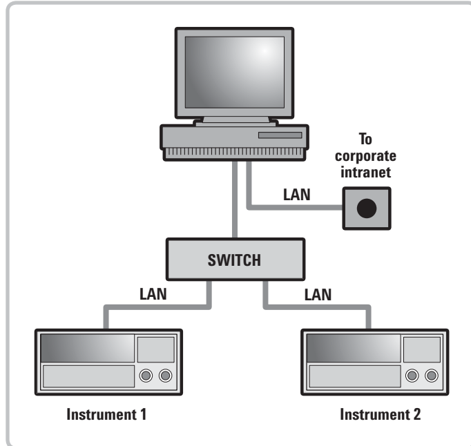
Figure 3. A PC configured with two LAN cards enables the creation of a private, protected network that can also access the corporate intranet
